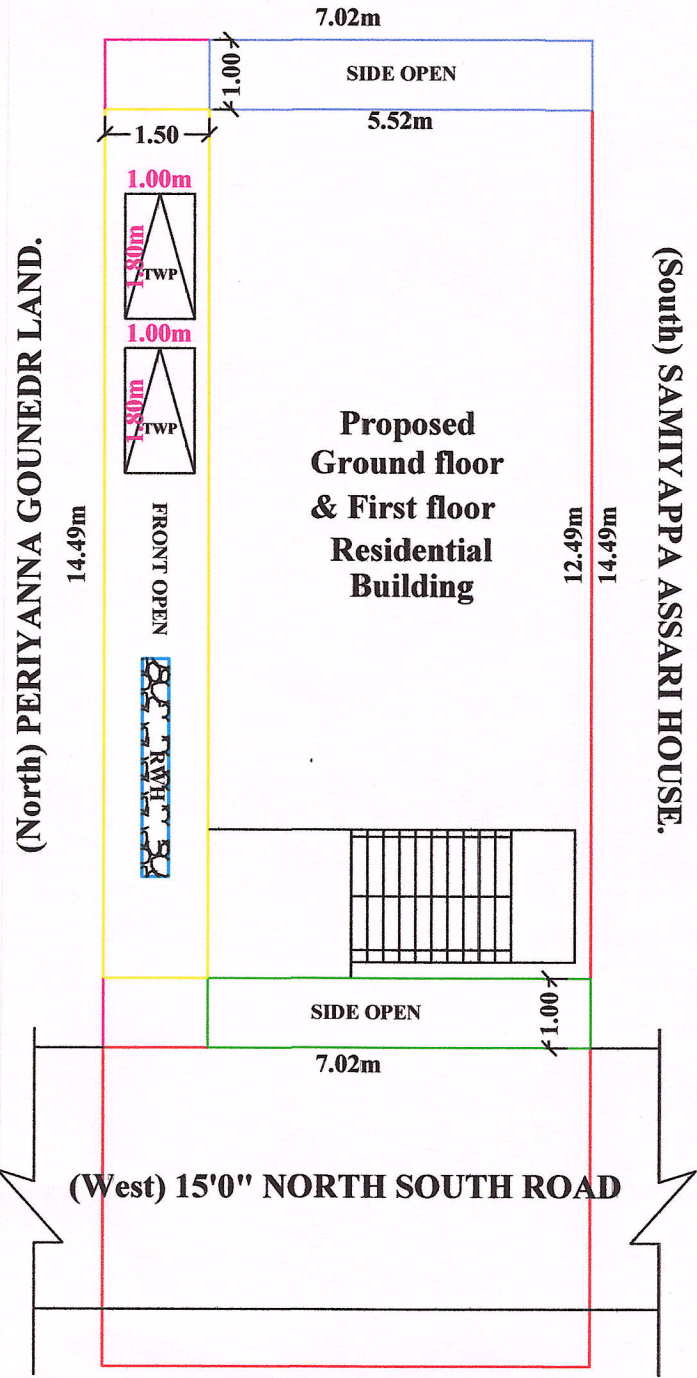
SITE PLAN
