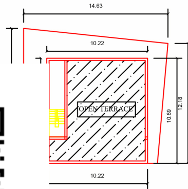
OPEN TERRACE
