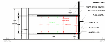
SECTION ON B-B
