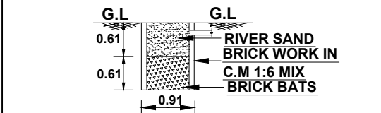
. SECTION ON RAIN WATER COLLECTION TUB .
