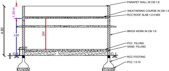
SECTION ON - "SR"
