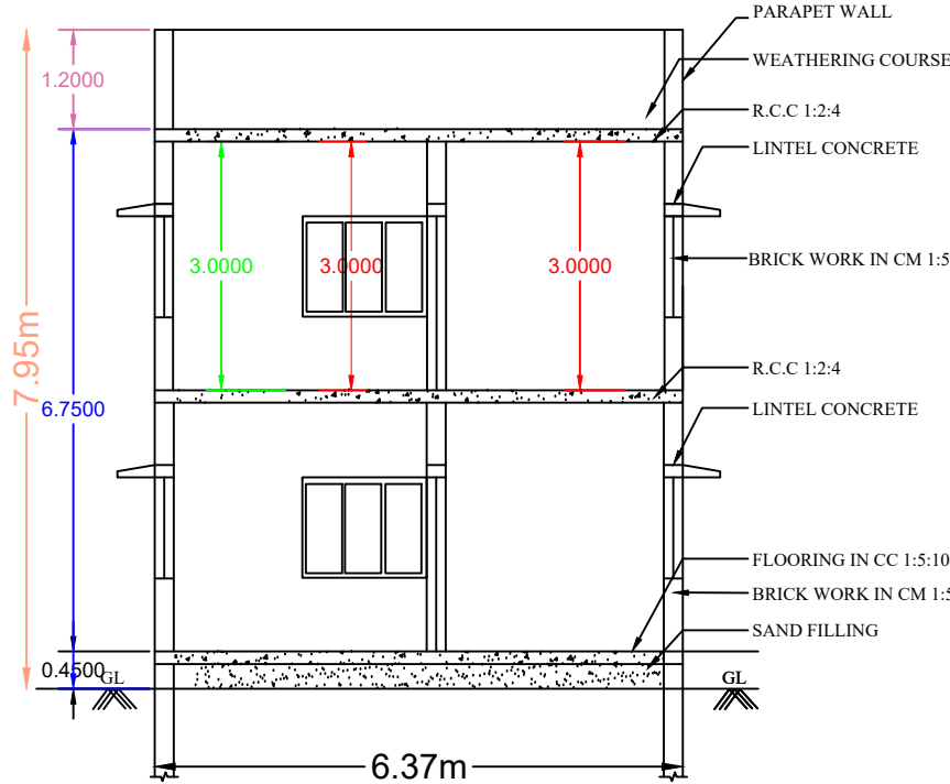
SECTION AB
