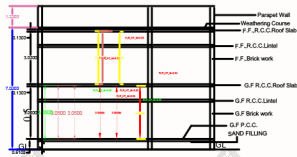
SECTION ON B-B
