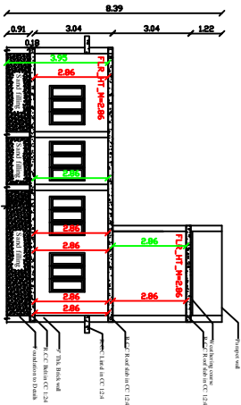
SECTION RCC
