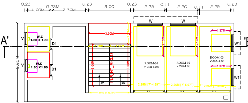
PRO. FIRST FLOOR PLAN.
