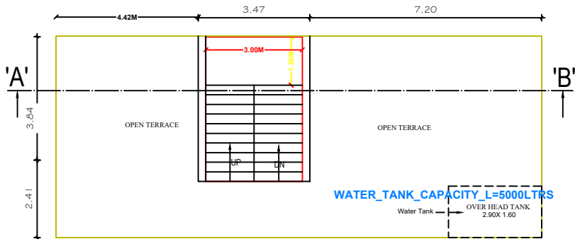
PRO. SECOND FLOOR PLAN.
