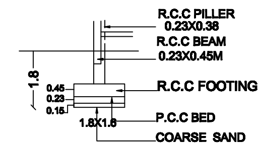
FOUNDATION DETAILS
