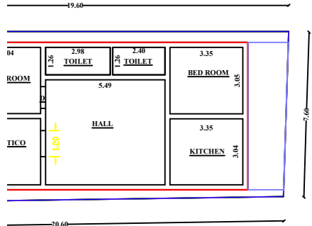
EXISTING GROUND FLOOR
