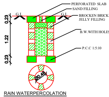
RAIN WATERPERCOLATION
