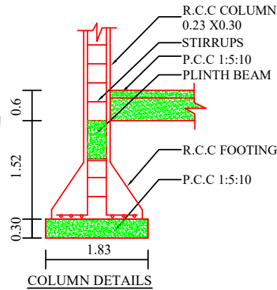
COLUMN DETAILS
