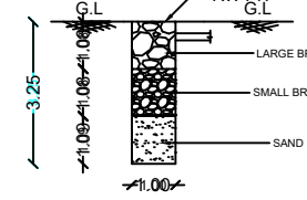
SECTION OF RAIN WATER HARVESTING PIT
