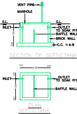
PLAN SEPTICTANK
