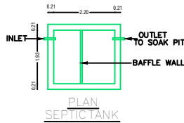
PLAN SEPTICTANK
