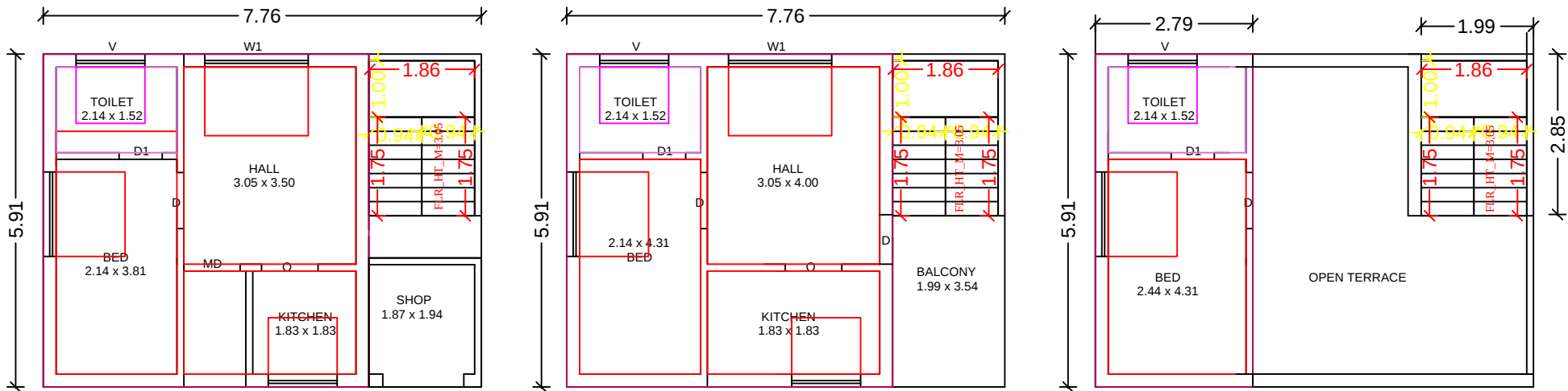
PRO. GROUND FLOOR PLAN
