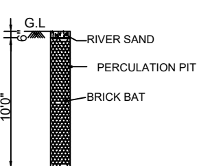
PERCOLATION PIT
