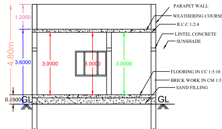
SECTION "AB"
