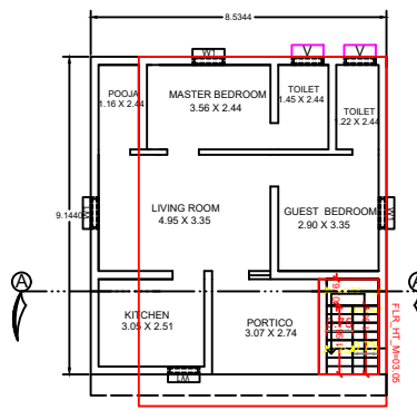
EXISTING GROUND FLOOR PLAN
