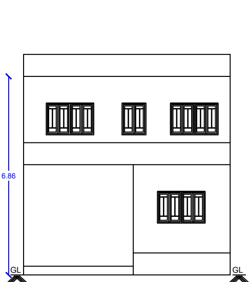
FRONT ELEVATION
