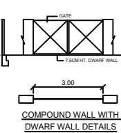
COMPOUND WALL WITH DWARF WALL DETAILS
