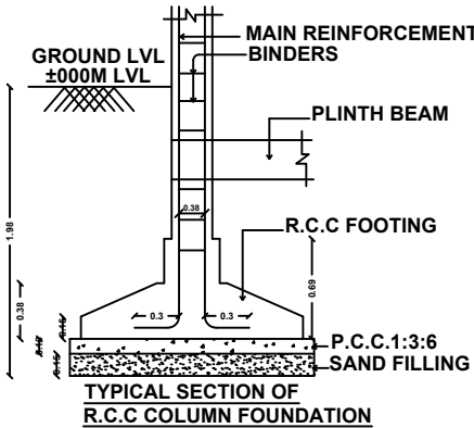
TYPICAL SECTION OF R.C.C COLUMN FOUNDATION
