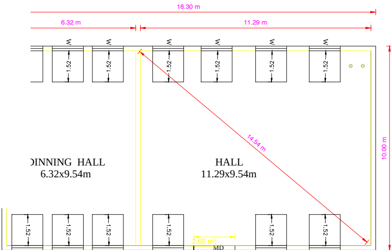
GROUND FLOOR PLAN ( ADDITIONAL CONSTRUCTION)
