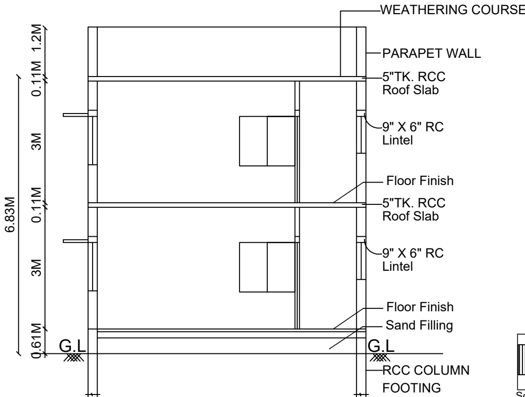
SECTION ON 'SP'
