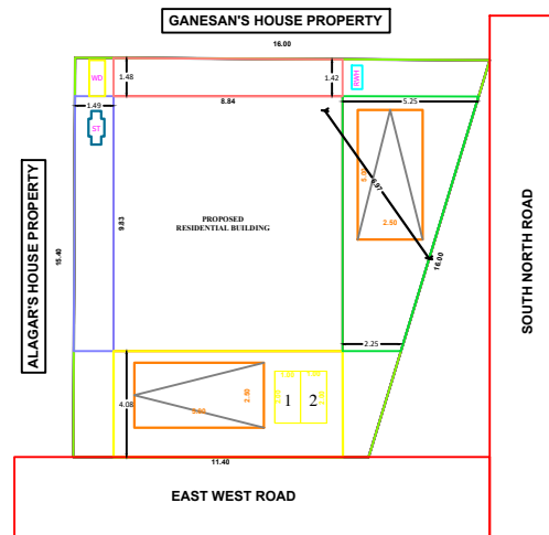
SITE PLAN
