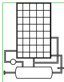
SOLAR SYSTEM
