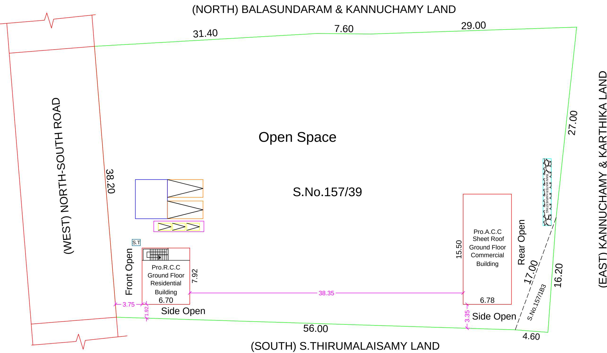
SITE PLAN
