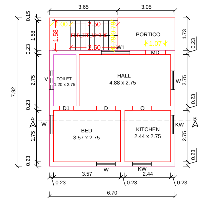
PRO.GROUND FLOOR PLAN BLOCK I -RESIDENTIAL
