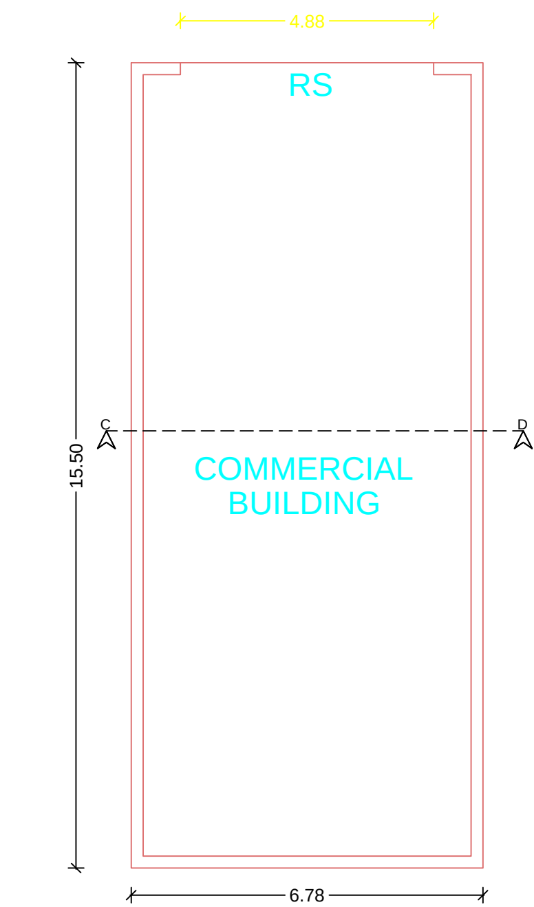
PRO.GROUND FLOOR PLAN BLOCK II -COMMERCIAL
