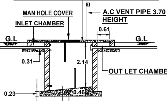
.SECTION ON SEPTIC TANK .
