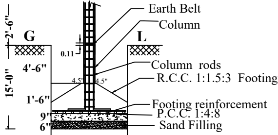
FOUNDATION DETAIL (NTS)
