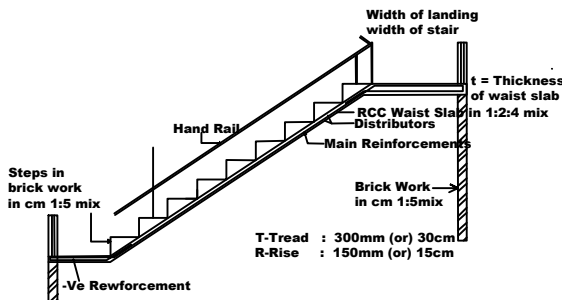
TYPICAL CROSS SECTION OF STAIRCASE DETAILS (NOT TO SCALE)
