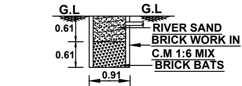
. SECTION ON RAIN WATER COLLECTION TUB .
