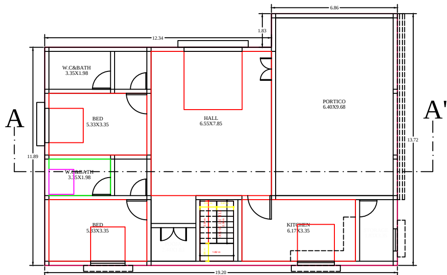
EXISTING GROUND FLOOR RESIDENTIAL BUILDING APPROVAL NO:33/2019, DATE :04.09.2019
