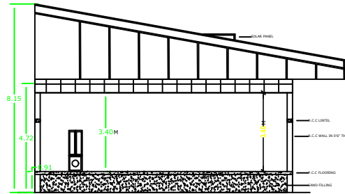
SECTION ON K-S
