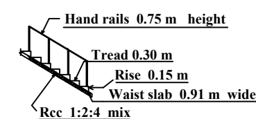
Staircase Details
