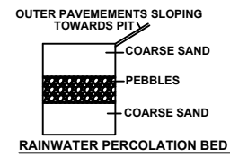
RAINWATER PERCOLATION BED
