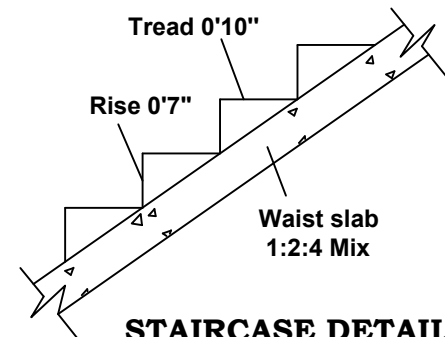
STAIRCASE DETAILS (NOT TO SCALE)
