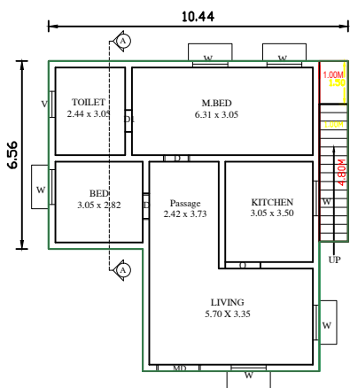
EXI. GROUND FLOOR PLAN
