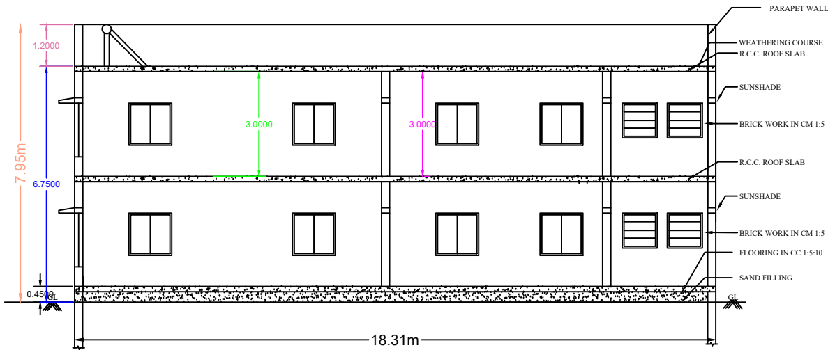
SECTION AB
