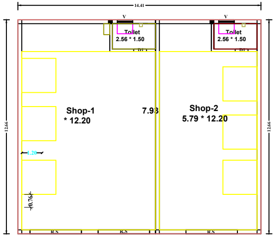
PROPOSED GROUND FLOOR - SHOP BUILDING
