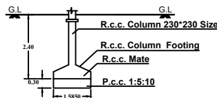
Foundation Details
