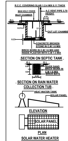
SOLAR WATER HEATER
