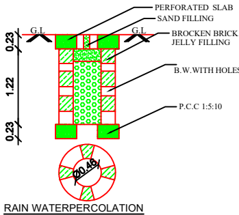
RAIN WATERPERCOLATION
