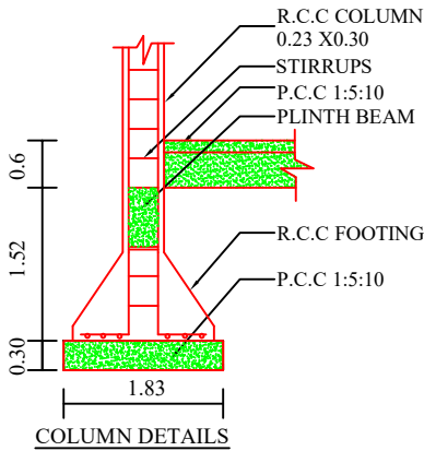
COLUMN DETAILS
