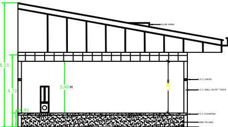
SECTION ON K-S
