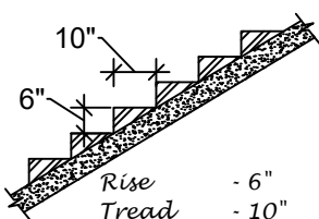
STAIR DETAIL
