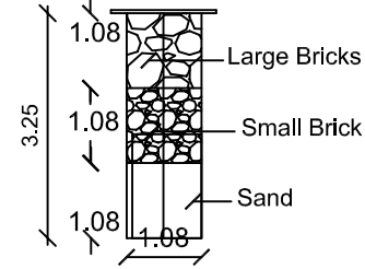
SECTION OF RAIN WATER
