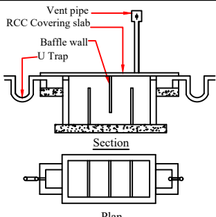
Section
