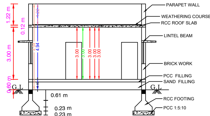
SECTION ON KA
