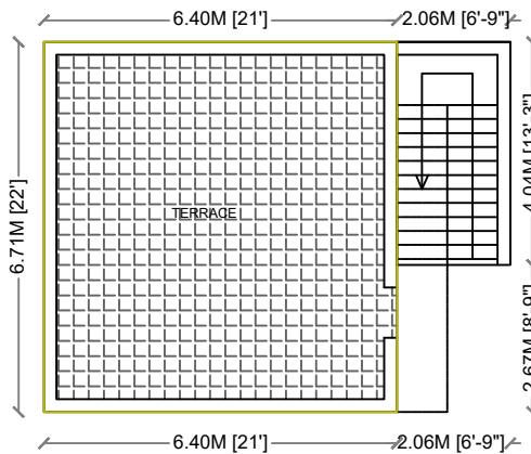
TERRACE PLAN
