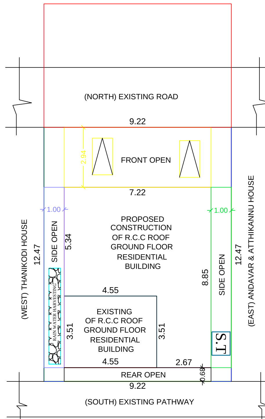
SITE PLAN
