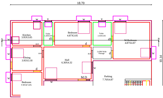
KEY PLAN
