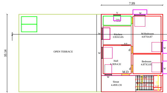
FIRST FLOOR PLAN AND TERRACE FLOOR PLAN
