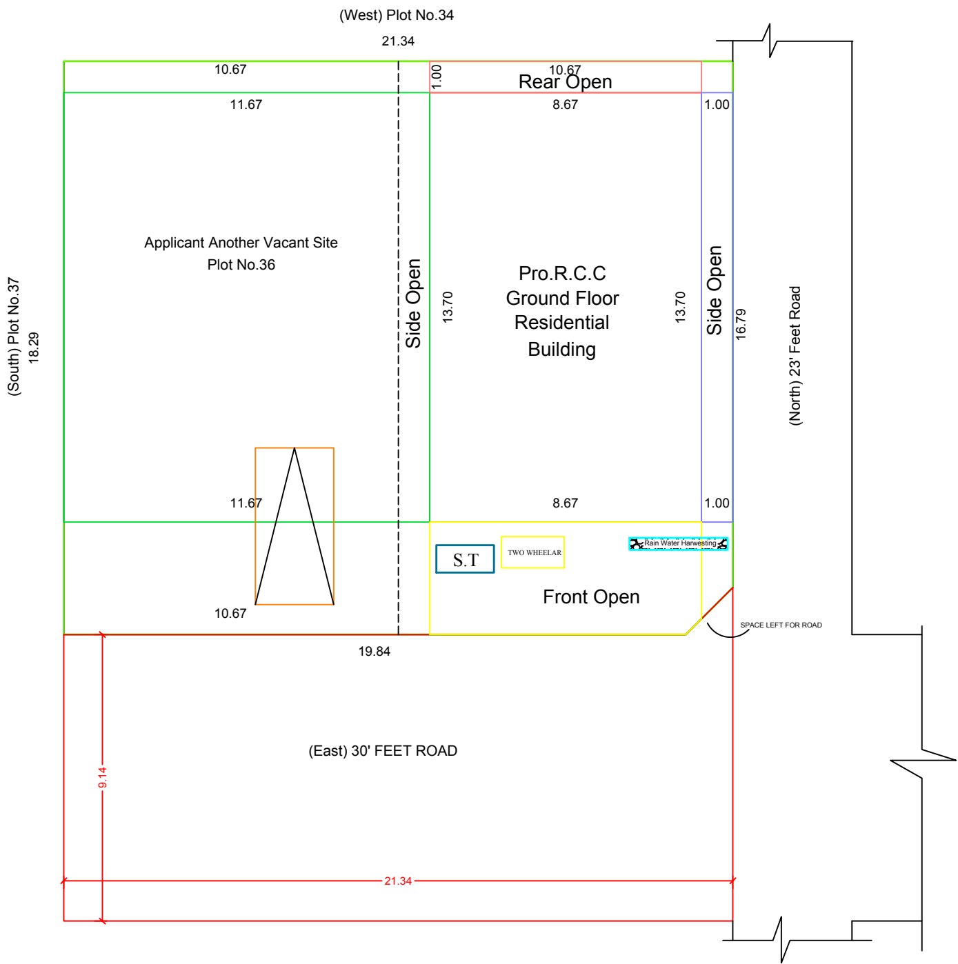
SITE PLAN
