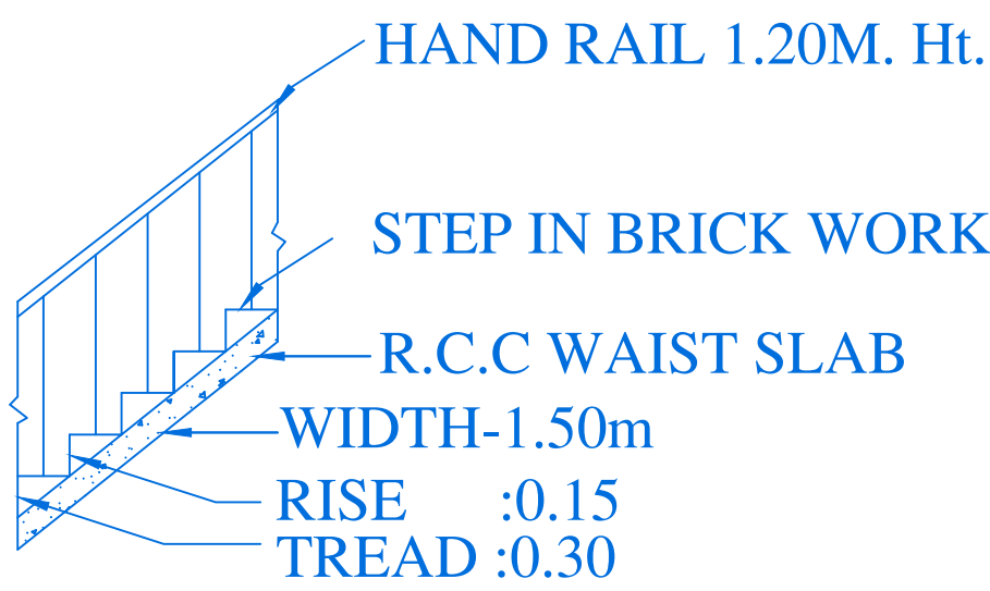
STAIR DETAIL
