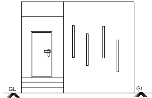
FRONT ELEVATION (EAST FACING)
