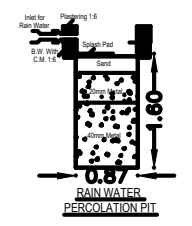
RAINWATER PERCOLATION PIT
