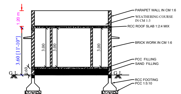
SECTION - "SR"
