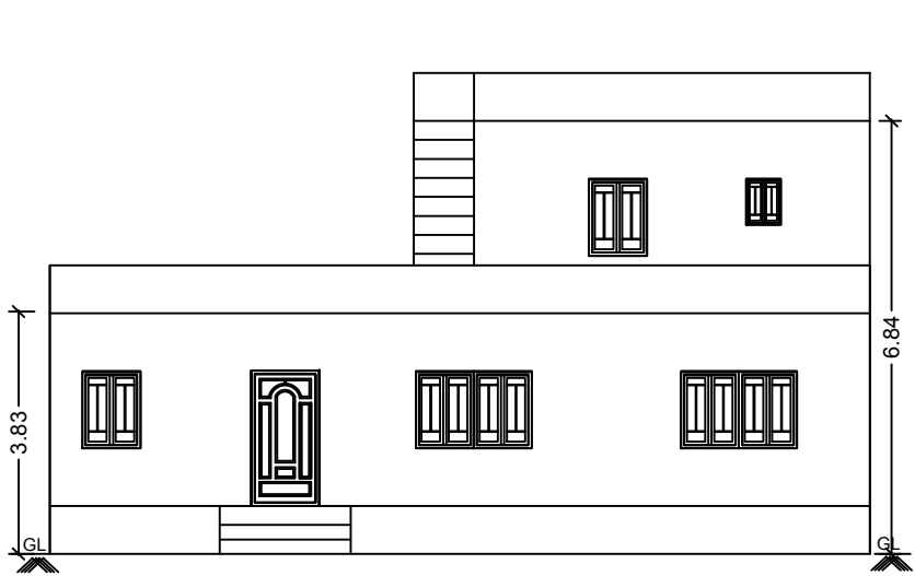
FRONT ELEVATION (NORTH FACING)
