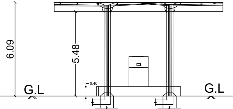
SECTION ON 'B'-B' (CANOPY)
