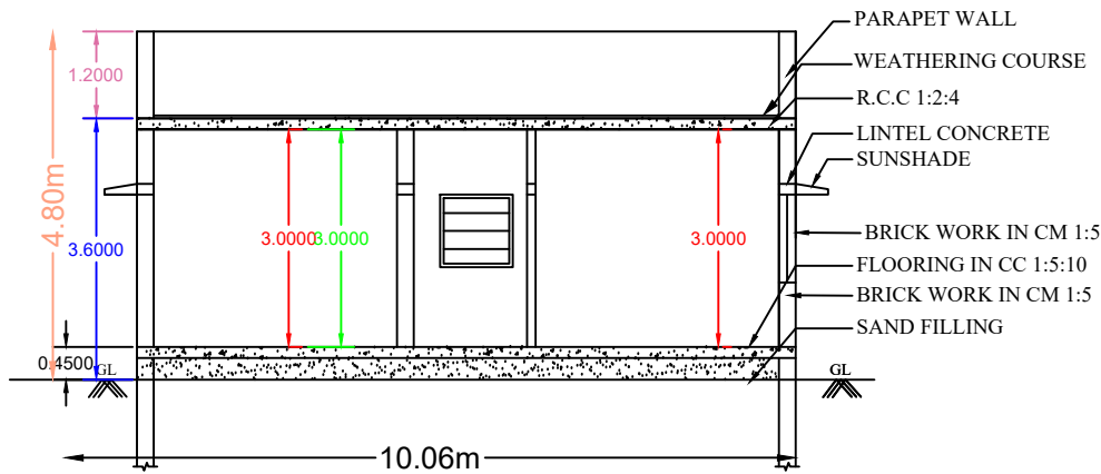
SECTION AB
